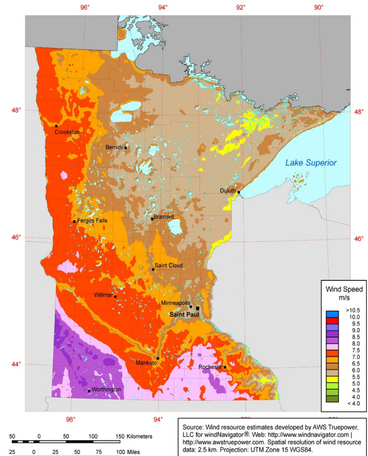
Minnesota - Annual Average Wind Speed at 80 m
